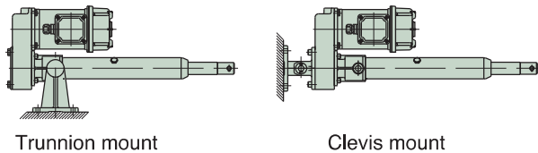
Fig. 1 Installation method
