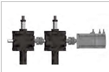
Two jacks in synchronized operation (Lifting)
