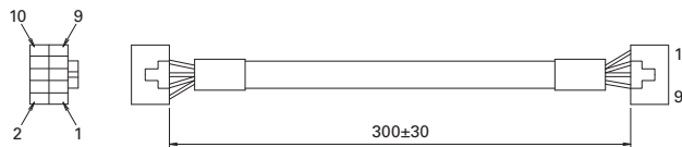
Wiring between connectors
