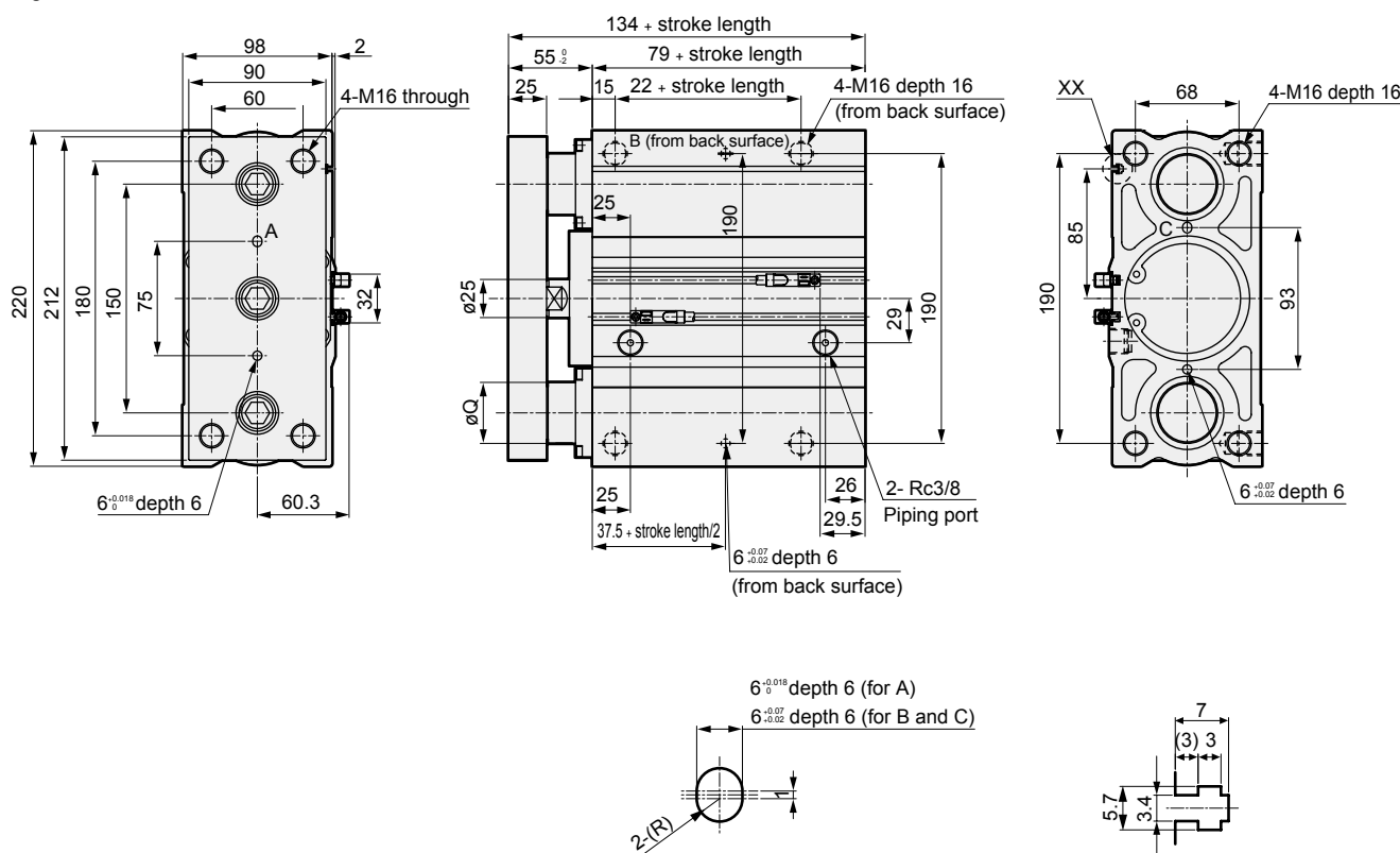
Slot dimensions for A, B and C
