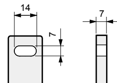
Enlarged view of bracket section
