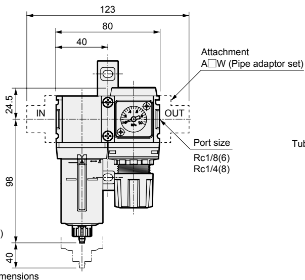
Pressure gauge attached optional dimensions table
