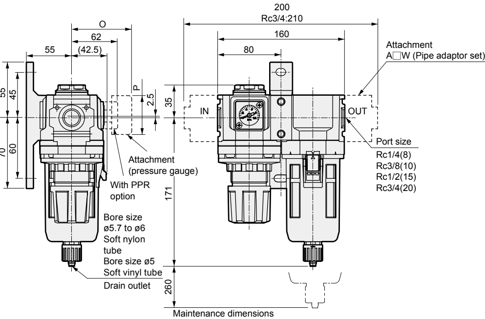
Pressure gauge attached optional dimensions table
