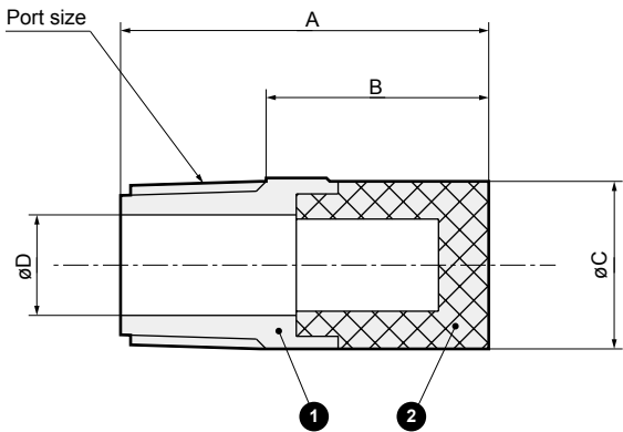
Cross-section A-A
